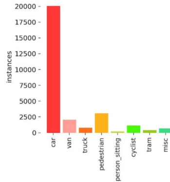
Figure 4: Label instances in KITTI dataset
