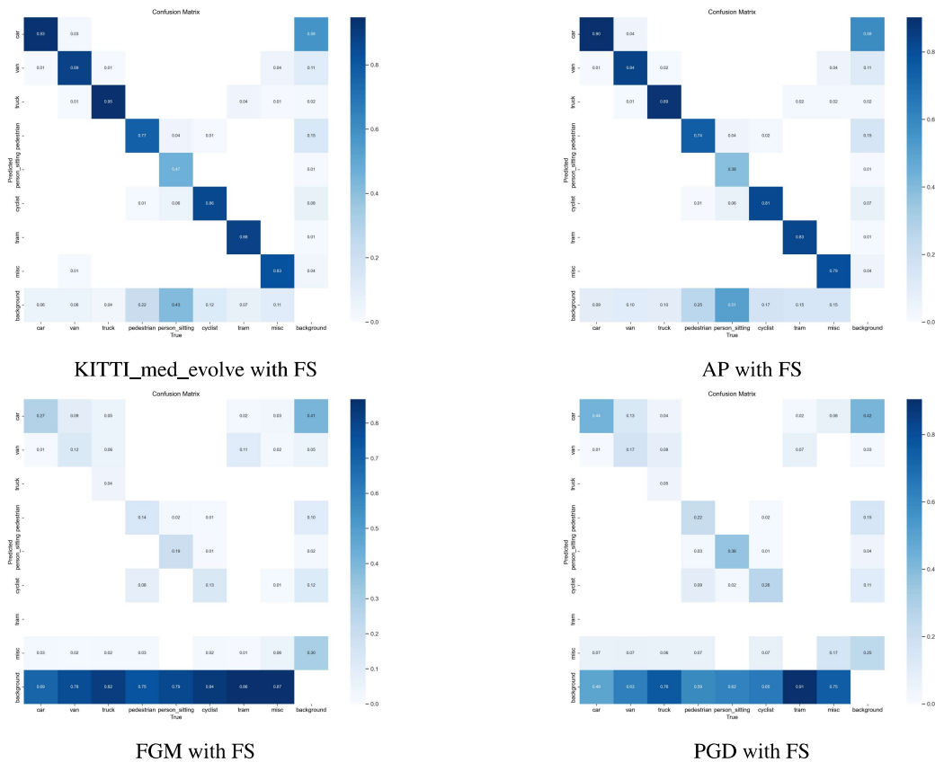
Figure 26: Attack confusion matrixes with FS
