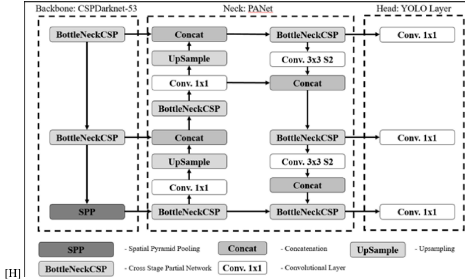
Figure 1: YOLOv5 architecture [28].
