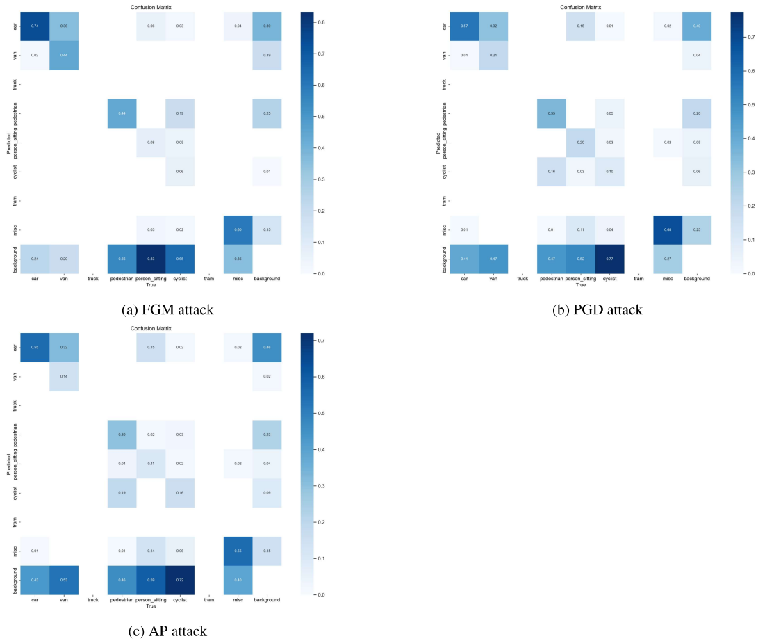
Figure 29: Attack confusion matrixes with SS in real-life environment
