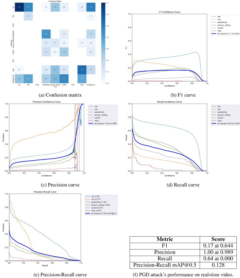
Figure 19: PGD video result metrics
