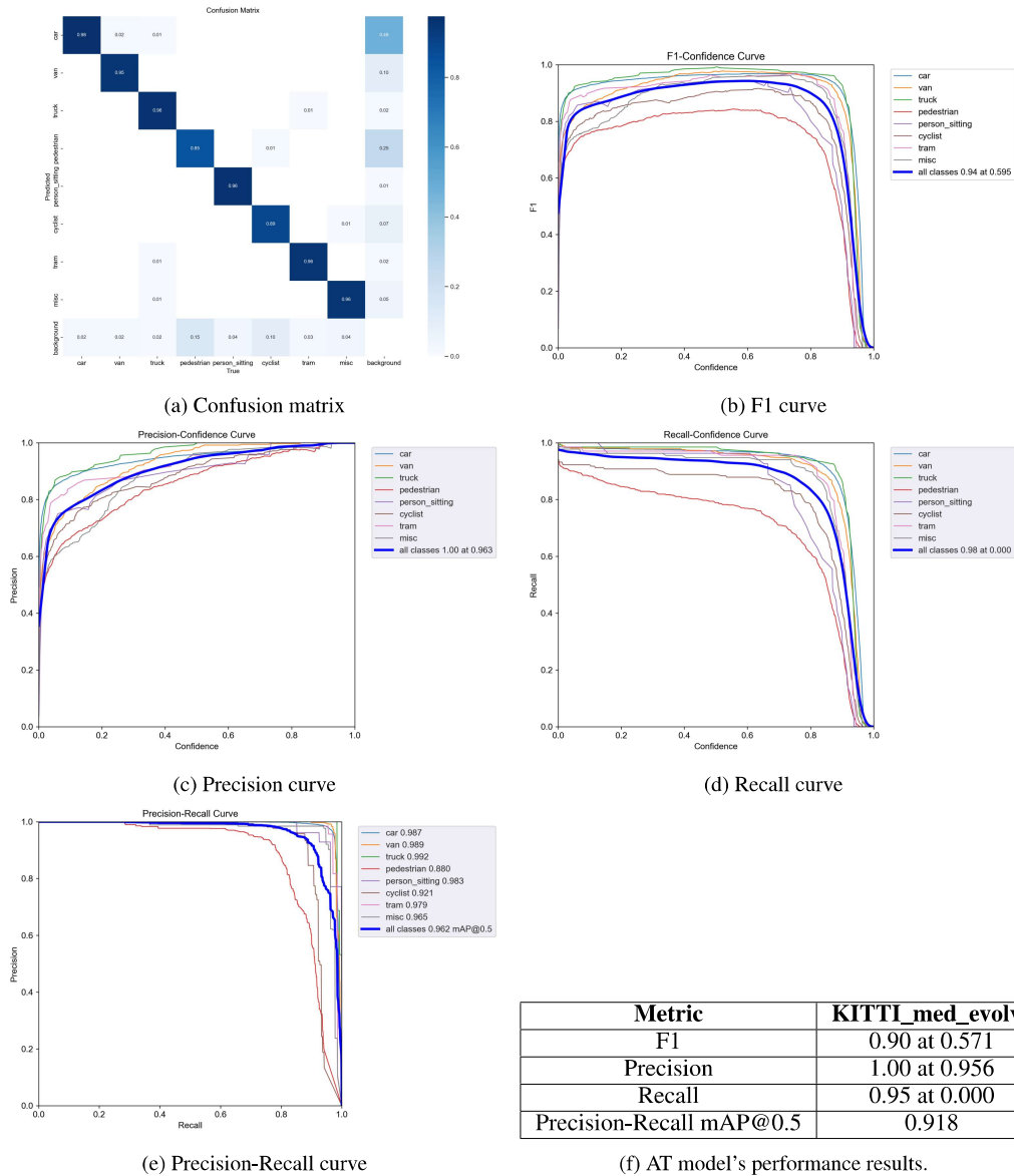
Figure 23: AT result metrics
