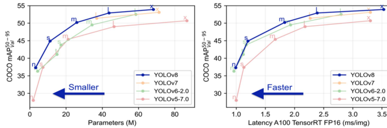
Figure 2: YOLO model comparison [13].
