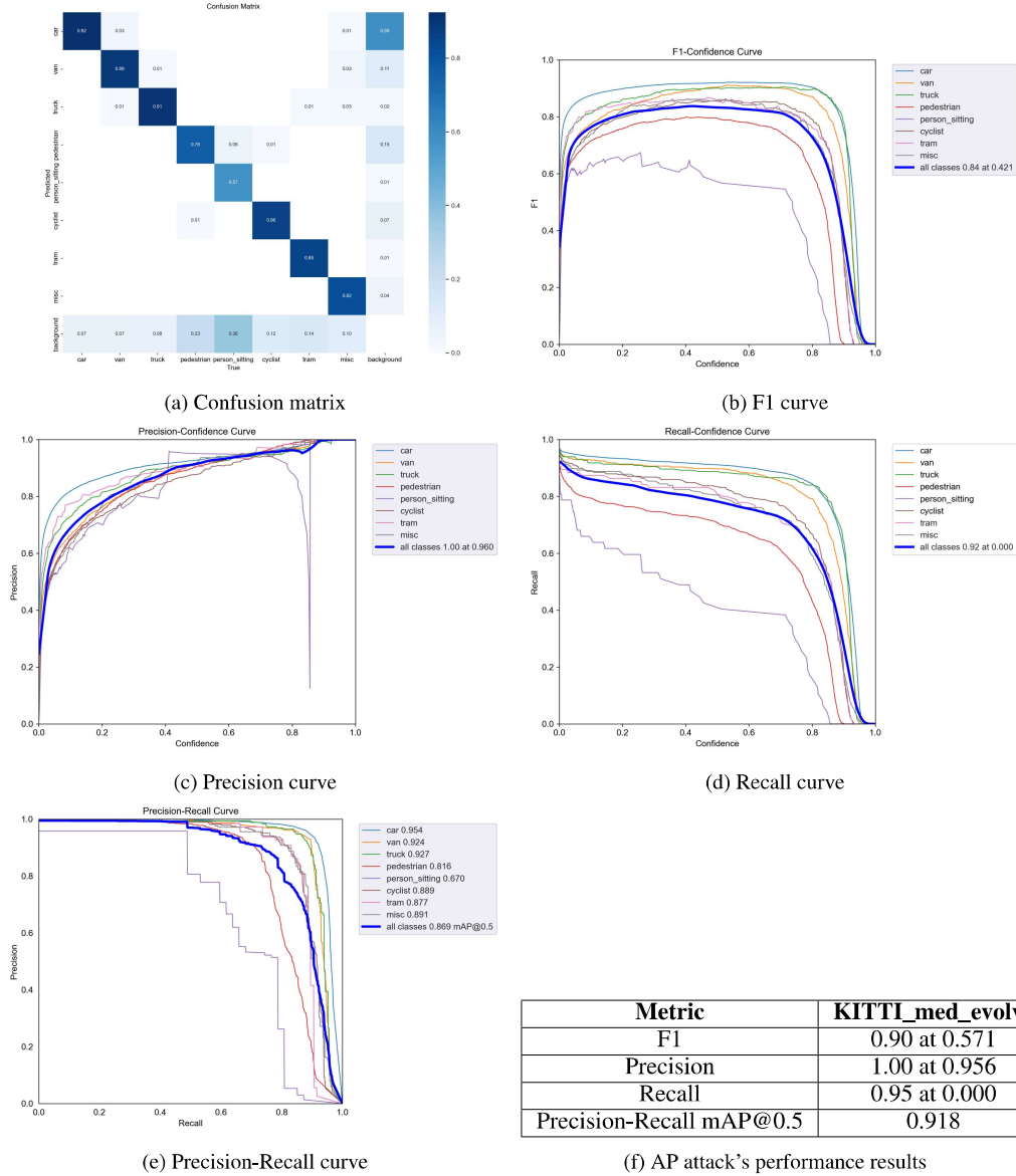
Figure 20: AP testing result metrics
