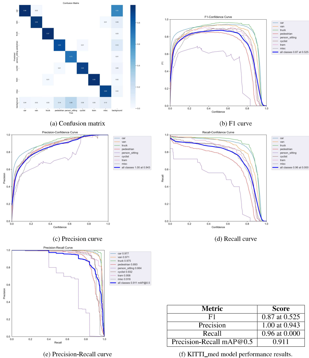
Figure 14: KITTI_med result metrics
