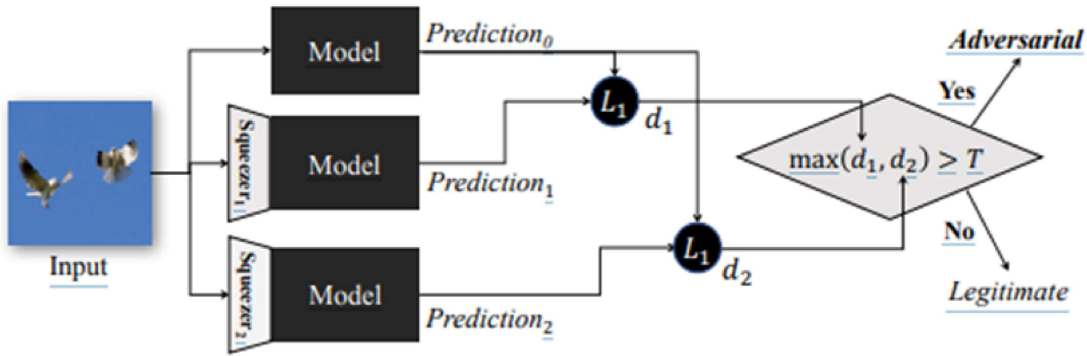
Figure 6: Feature squeezing as portrayed in the paper [34].
