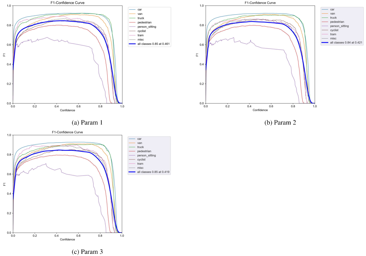
Figure 9: AP attack with different parameters
