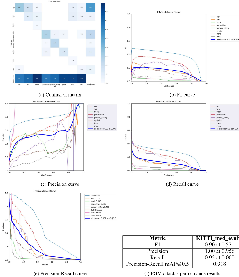
Figure 16: FGM testing result metrics
