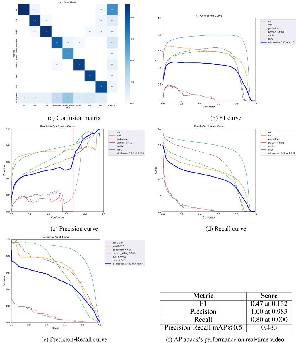
Figure 21: AP video result metrics
