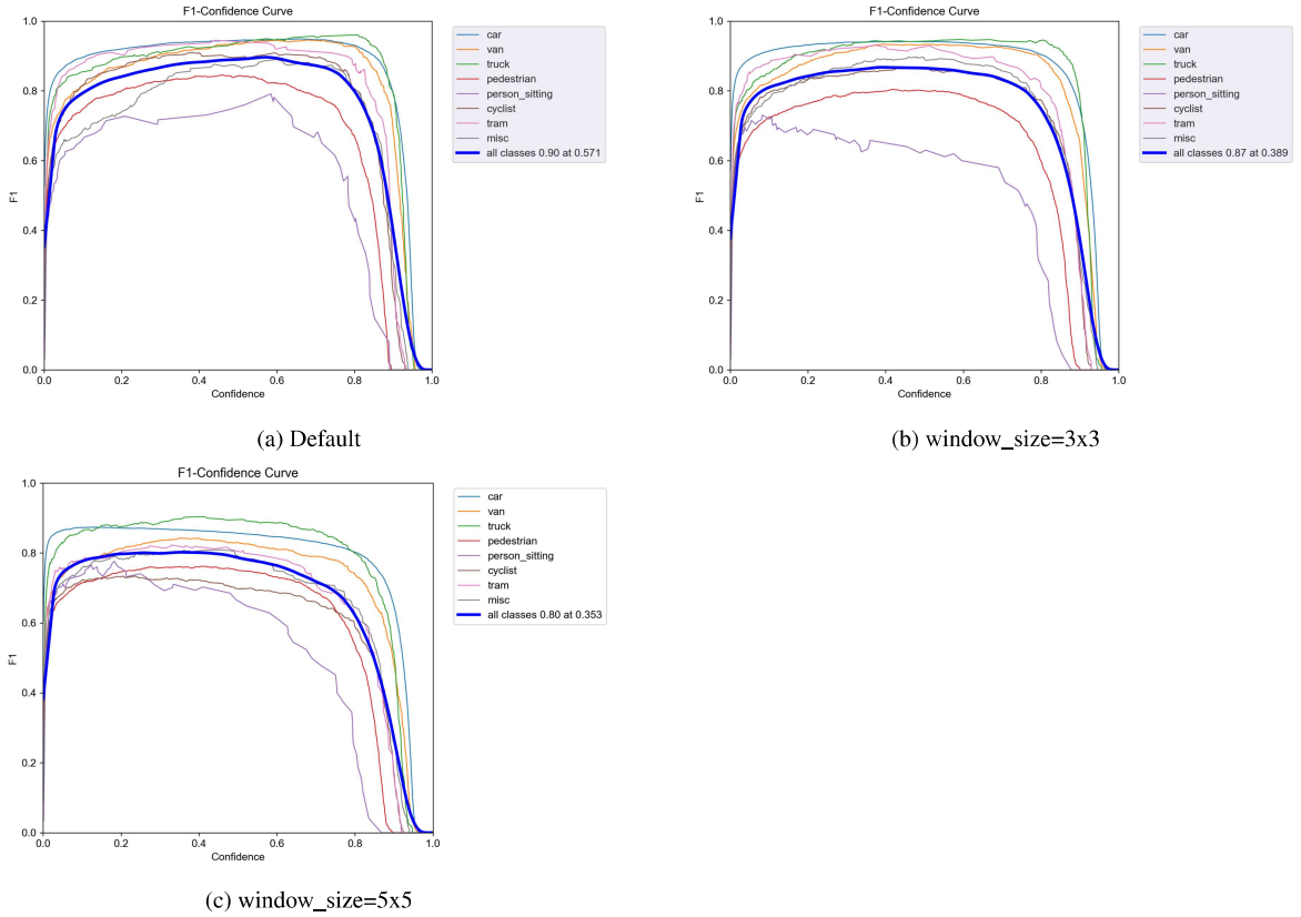
Figure 12: SS defence with different window_size
