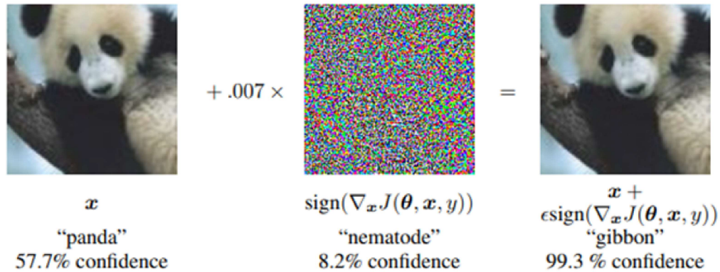
Figure 5: example of FGM attack.
