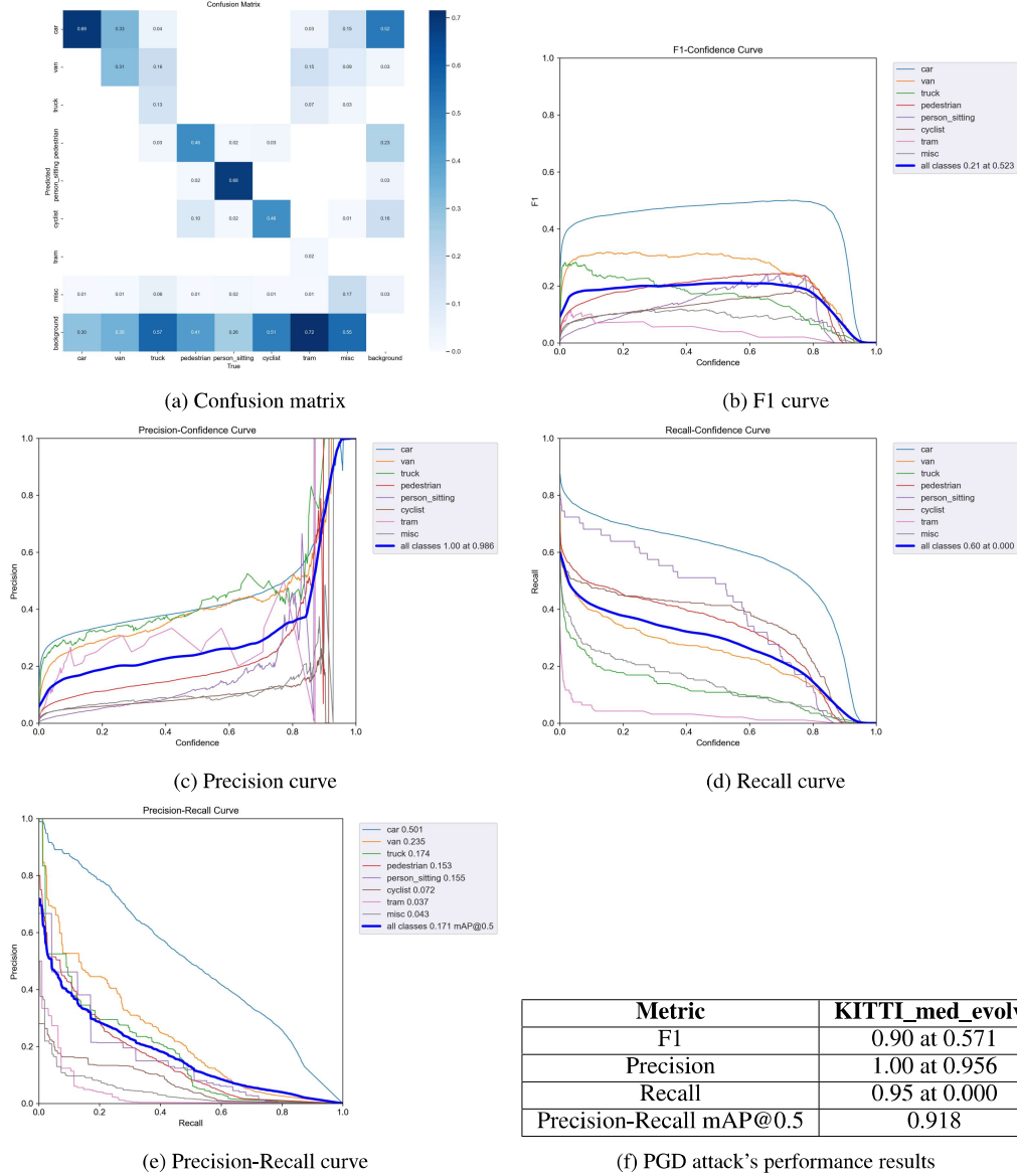
Figure 18: PGD testing result metrics
