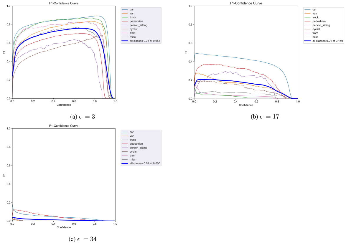
Figure 7: FGM attack with different \epsilon values
