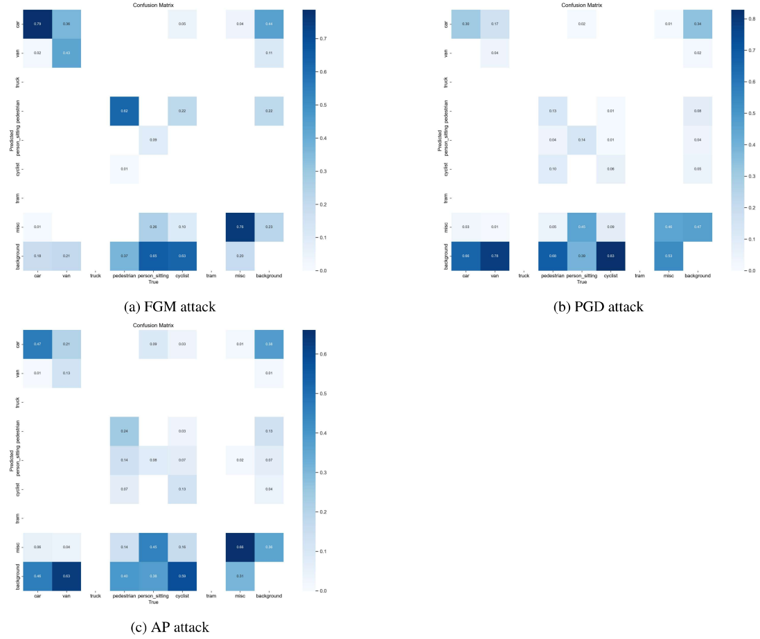
Figure 27: Attack confusion matrixes with FS in real-life environment
