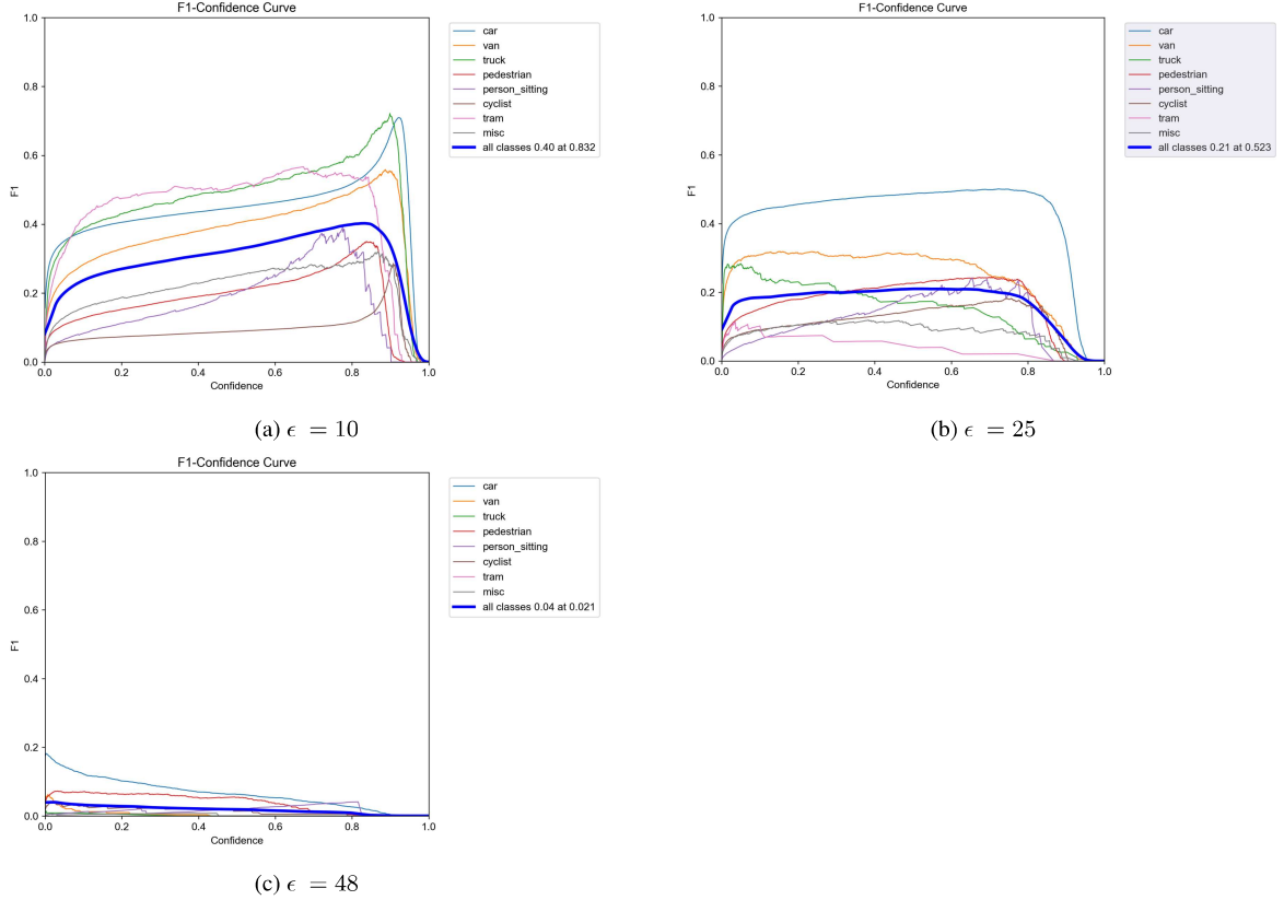
Figure 8: PGD attack with different \epsilon values
