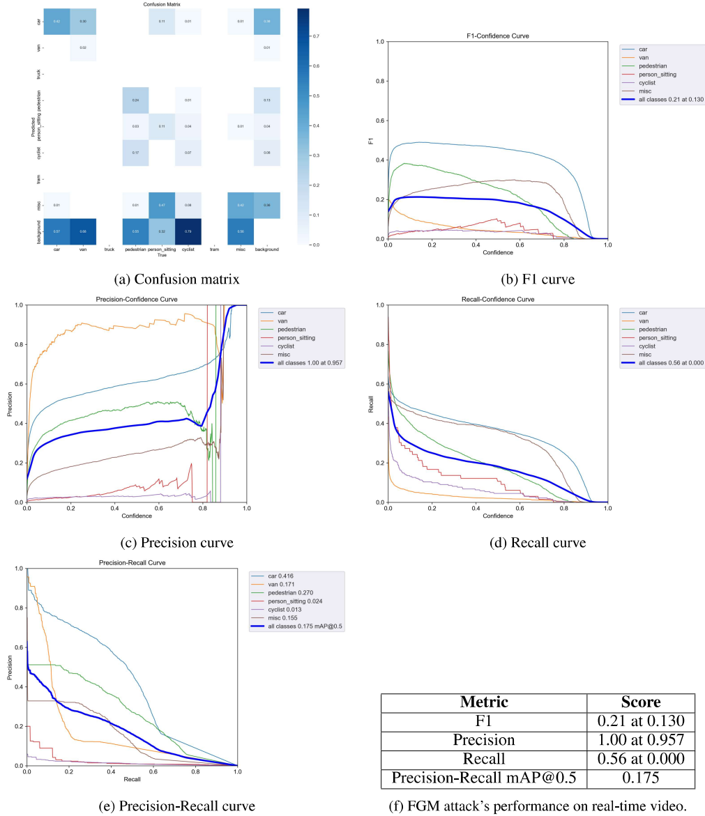
Figure 17: FGM video result metrics
