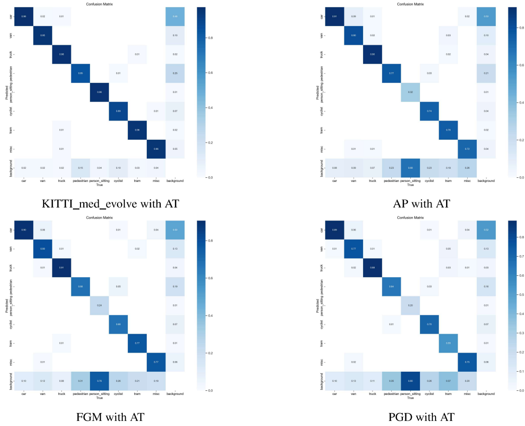
Figure 24: Attack confusion matrixes with AT
