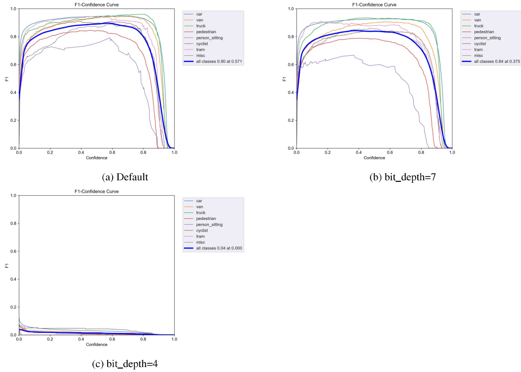
Figure 10: FS defence with different bit_depth
